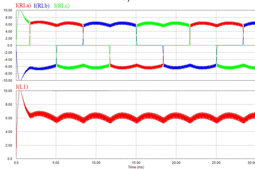
Figure 2. a) Three-phase on-line UPS system with an uncontrolled rectifier, b) Current through inductor L_1 and input phase currents I(RL_a) , I(RL_b) , and I(RL_c)
