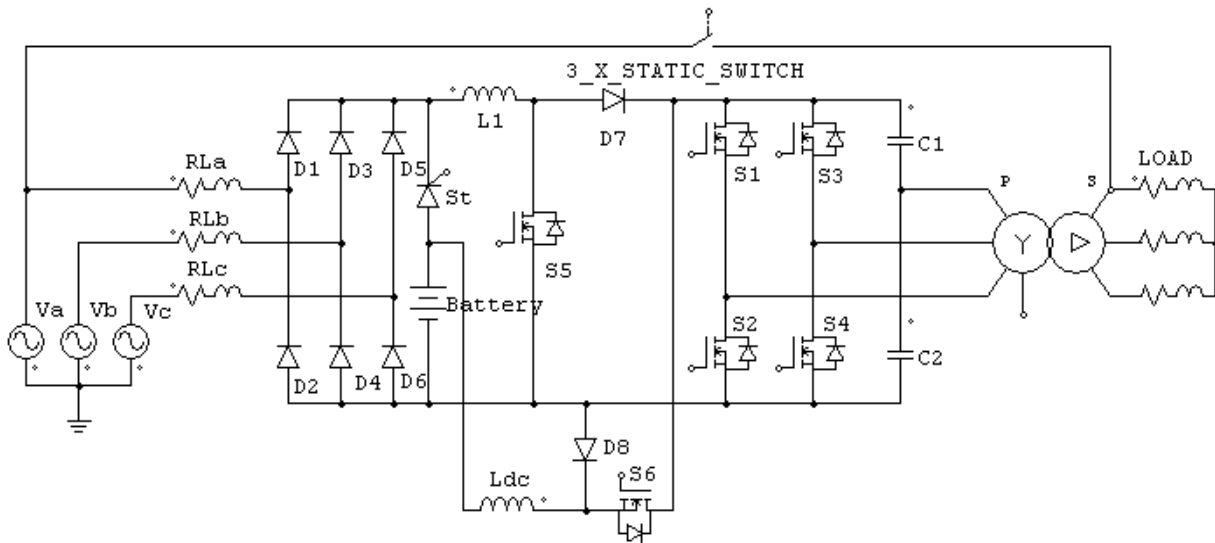
Figure 3. Three-phase on-line UPS system reduced number of switches.
