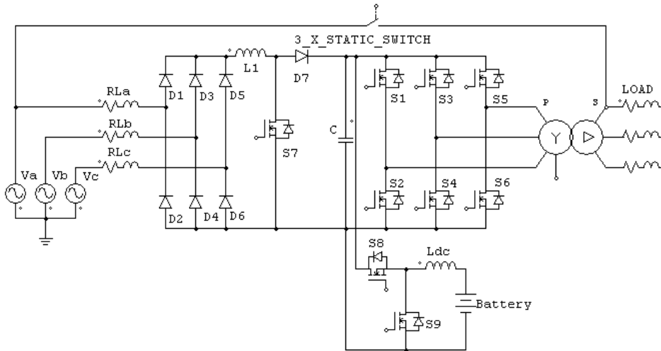
Figure 1. a) Three-phase on-line UPS system with a controlled rectifier, b) Input phase voltages V_a , V_b , V_c , and input phase currents I(RL_a) , I(RL_b) , and I(RL_c)
