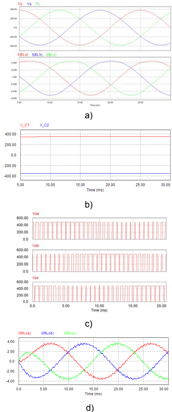
Figure 4. Simulation results for normal mode of operation: a) Input phase voltages V_a , V_b , V_c , and input phase currents I(RLa) , I(RLb) , and I(RLc) , b) DC-link voltages for each capacitor C_1 and C_2 , c) output phase voltages V_{oa} , V_{ob} , and V_{oc} , d) load phase currents I(RLoa) , I(RLob) , and I(RLoc) .
