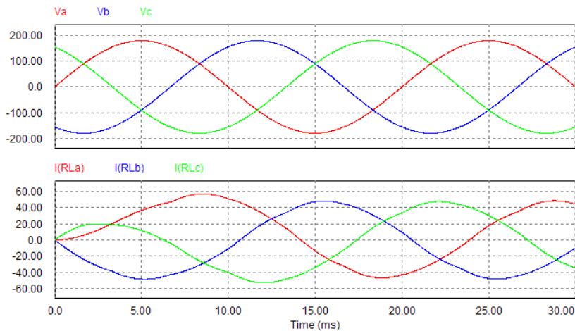
Figure 1. a) Three-phase on-line UPS system with a controlled rectifier, b) Input phase voltages V_a , V_b , V_c , and input phase currents I(RL_a) , I(RL_b) , and I(RL_c)
